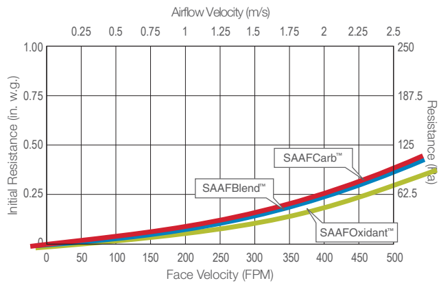
Initial Resistance vs. Face Velocity
