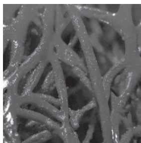
Heavily Loaded Air Entering Side Same magnification of heavily loaded pad illustrates the large holding capacity of each fibre. The open space between fibers continues to permit good airflow and allow paint to penetrate.
